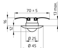
sensor head
