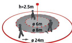
PD4N-M-DACO-PRO DALI-2
