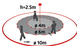
PD2N-M-DACO-PRO DALI-2
