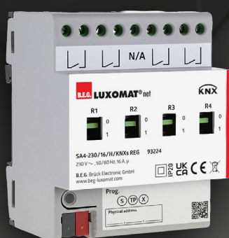
4 way switching actuator
