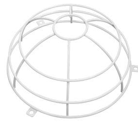
Wire basket BSK ( \varnothing 200 \times 90 mm) Art.No: 92199
