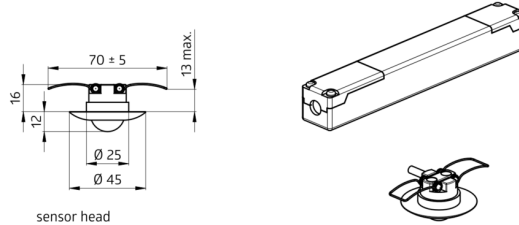
sensor head
