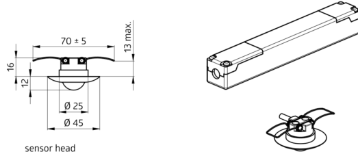
sensor head
